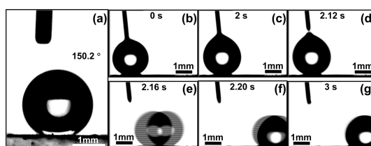
Figure 6. Superhydrophobic characteristics of the device surface. (a) Water droplet of 5 \mu\text{L} on the device surface, showing a contact angle of 150.2^\circ . (b–g) CCD images of the rolling off process of the water droplet on the device surface at different times.
