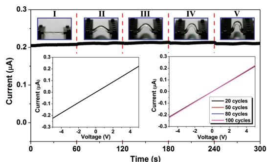
Figure 4. I – T curve of CNPs on PDMS substrate bent with different curvatures under a constant voltage. The upper insets labeled I, II, III, IV, and V demonstrate the five bending states. The lower left inset shows the I – V curve of CNPs without bending. The lower right inset records the I – V curve of CNPs on PDMS after 20, 50, 80, and 100 cycles of bending.
